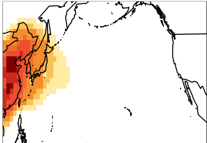
Gas phase
