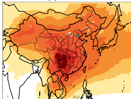
(c) Ozone
